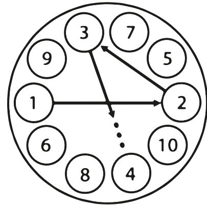
10-Bolt Hub
